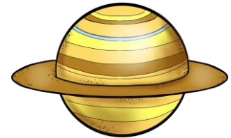
Satarn
