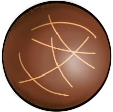
Mearcair
