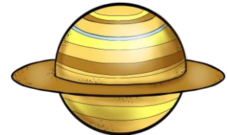
Saturn
