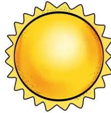
an ghrian
