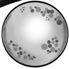
an ghealach
